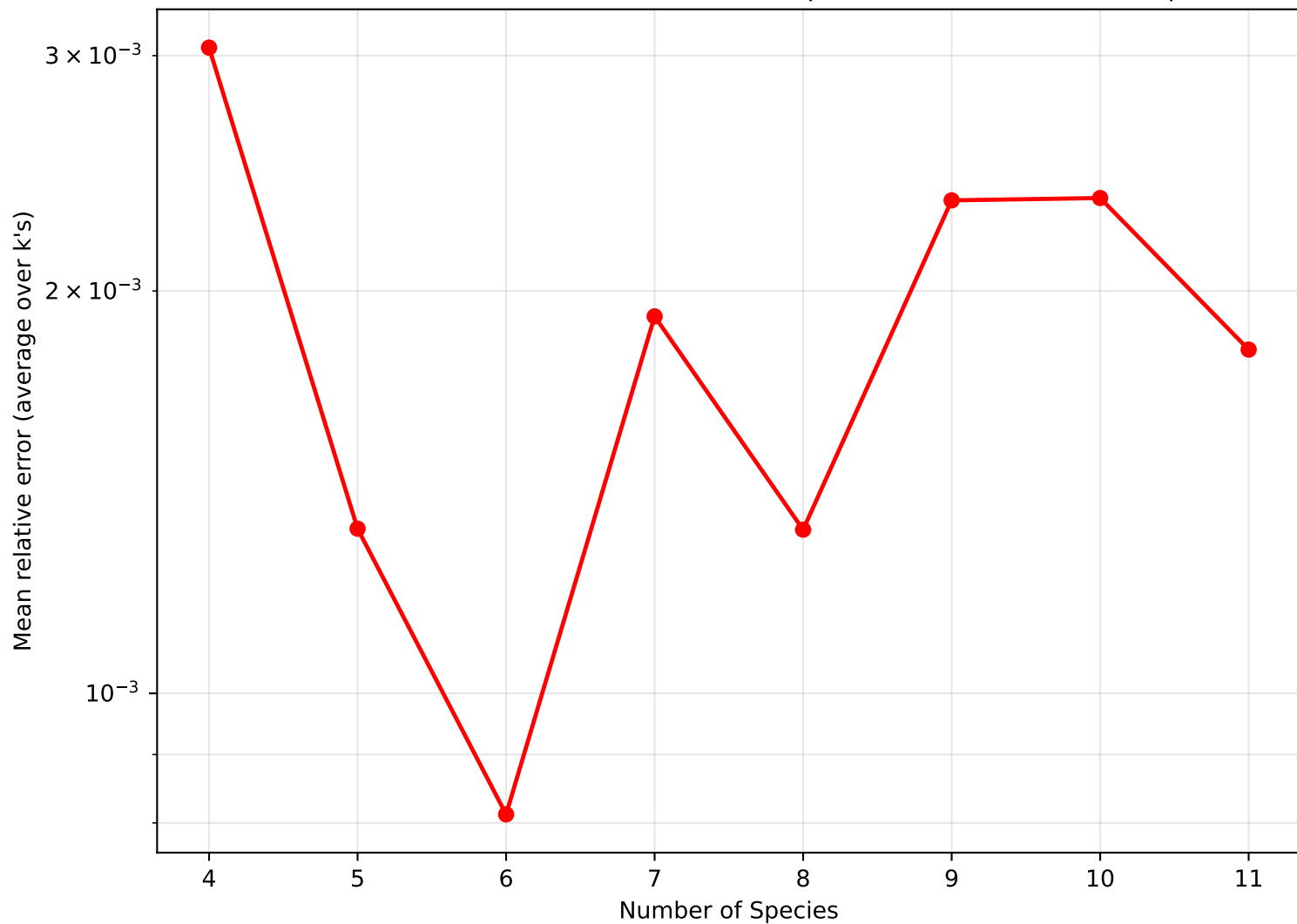
50, 50 — Mean relative error vs number of species (zoomed: 4 to 11 species)
